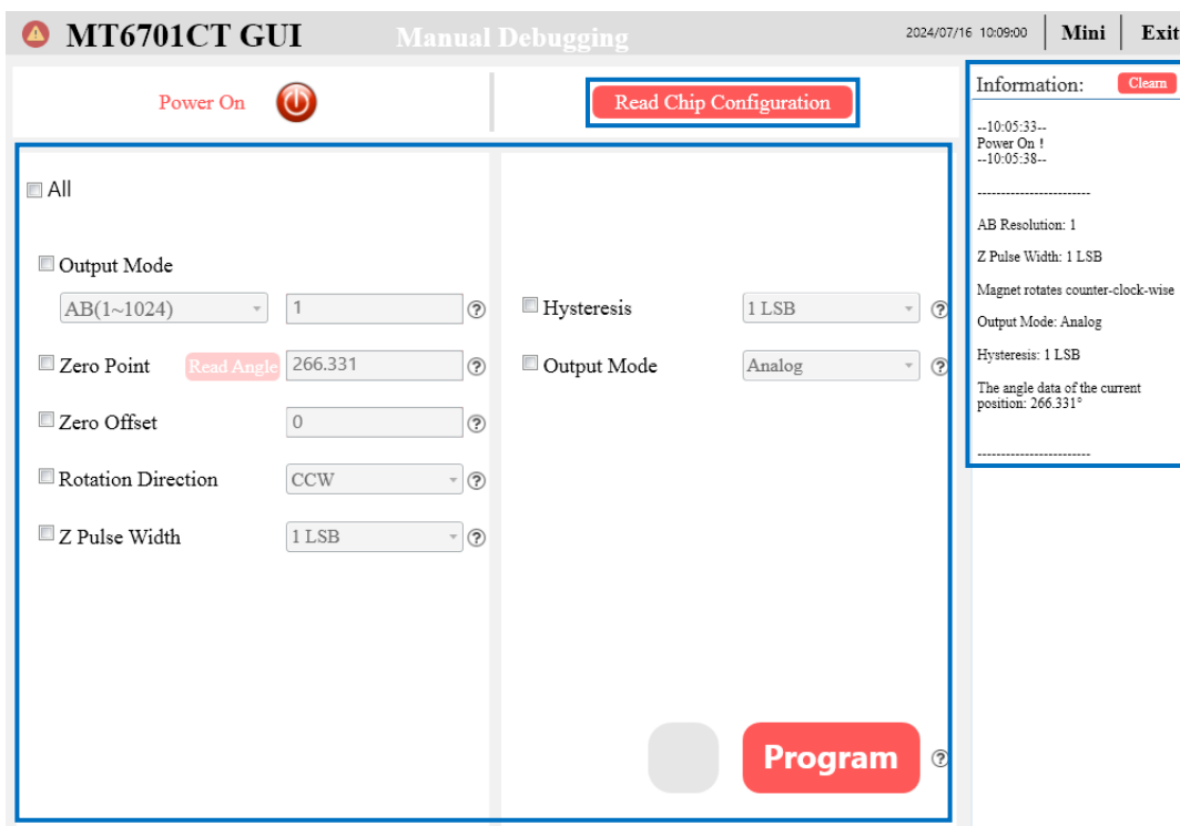
Figure 4.1.7 Read Chip Configuration
