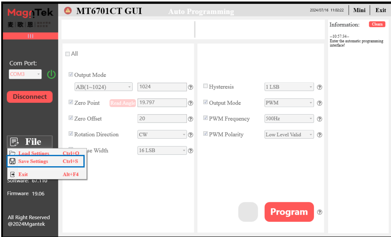
Figure 4.2.2 Set parameters and save the data
