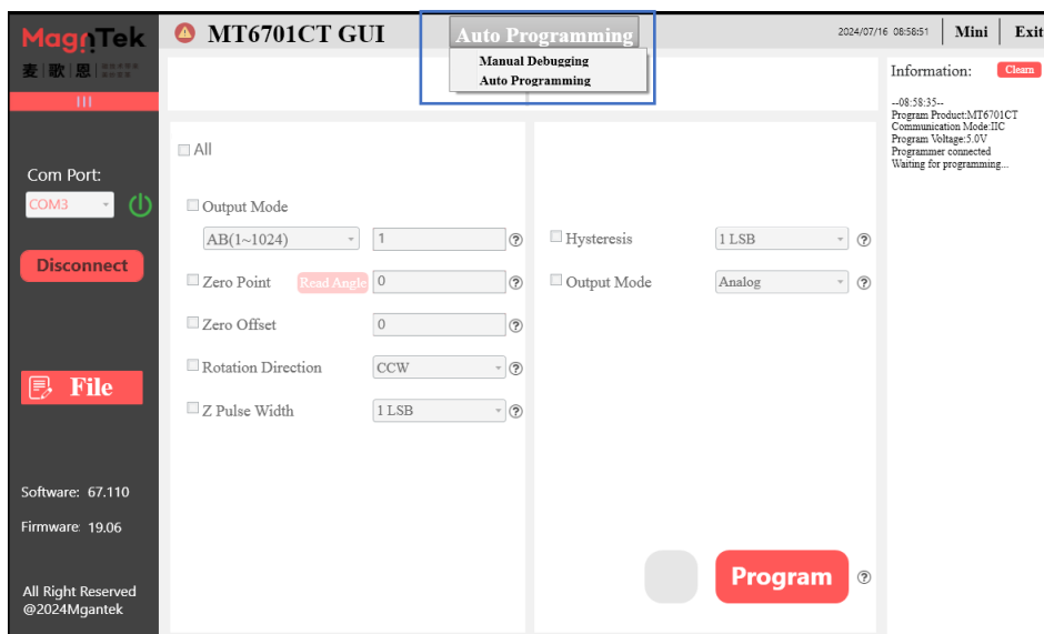
Figure 3.1.1 Program Interface Switch Selection
