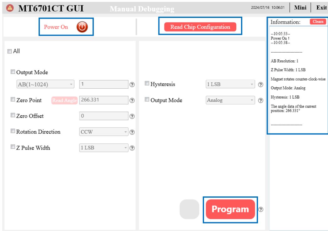
Figure 4.1.6 The interface state after chip power on
